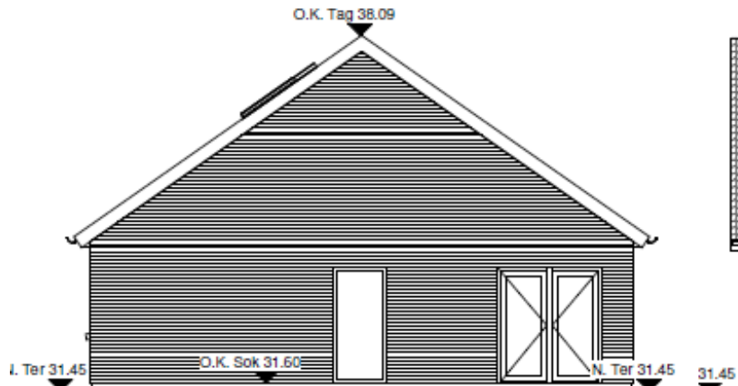
Facade mod Vest
